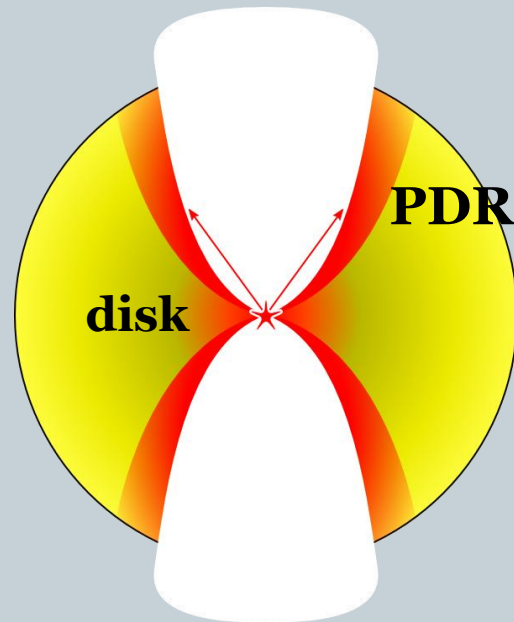
Cavity walls, disk surface: mid- J CO, low-velocity [O I]
