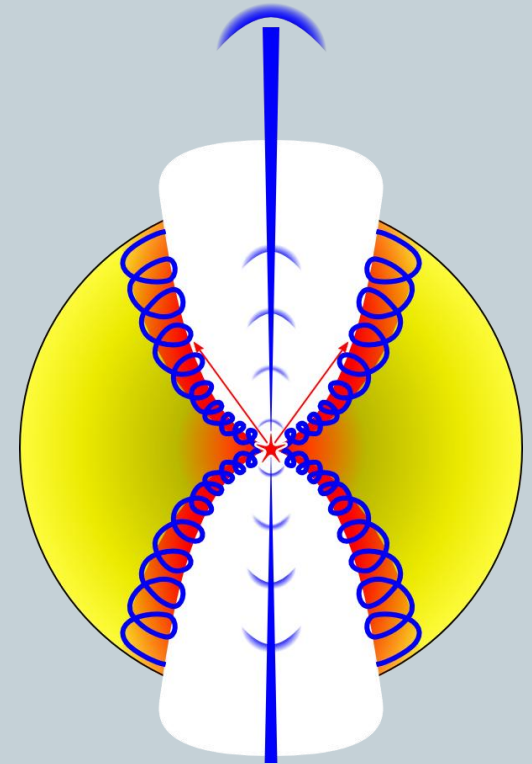
Outflow shocks: high- J CO, hot water (>100 K), high-velocity [O I]
