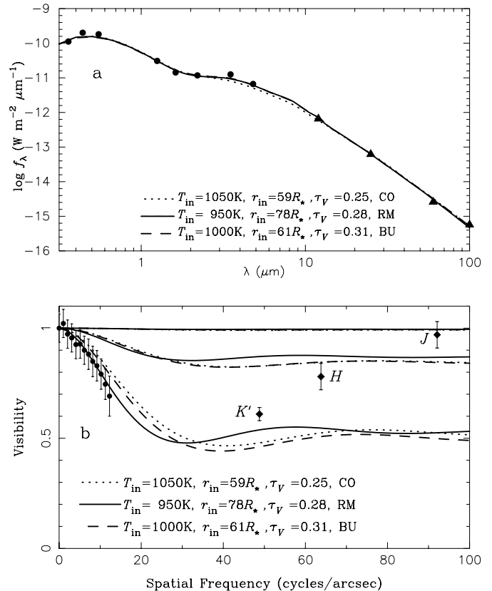
Fig. 2. Comparison of the observed SED and visibilities with SEDs and visibilities predicted by two-component models consisting of the central star and an optically thin dust shell, as described in Sect. 4.1. a) The filled circles represent the photometric data obtained five days after the IOTA observations. The filled triangles represent IRAS data. The three curves represent models with different opacities for amorphous carbon. RM: Rouleau & Martin (1991), CO: Colangeli et al. (1995), BU: Bussoletti et al. (1987). T_{\text{in}} is the temperature at the inner boundary ( r_{\text{in}} ) of the optically thin dust shell. \tau_V is the optical depth of a dust shell defined at 0.55 \mu\text{m} . b) The filled diamonds represent the J -, H -, and K' -band visibilities observed with IOTA. The filled circles represent the K' -band visibility obtained by speckle interferometry with the 6 m telescope at the Special Astrophysical Observatory, Russia (Paper I). For each of the RM, CO, and BU models, the predicted visibilities in the J -, H -, and K' bands are shown.
