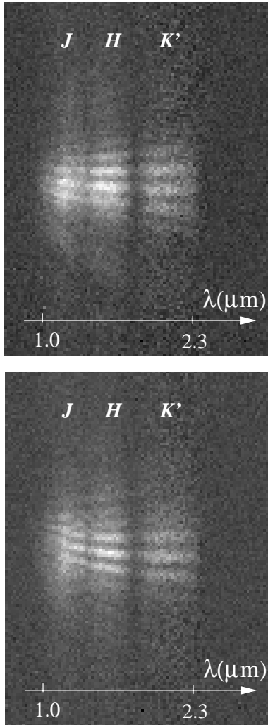
Fig. 1. Two consecutive interferograms of R CrB. The fringes are spectrally dispersed in the horizontal direction and are recorded simultaneously in the J , H , and K' bands, as shown in each panel. These three bands are separated by telluric absorption, which can be seen as vertical dark lanes between the J and H bands as well as between the H and K' bands.
