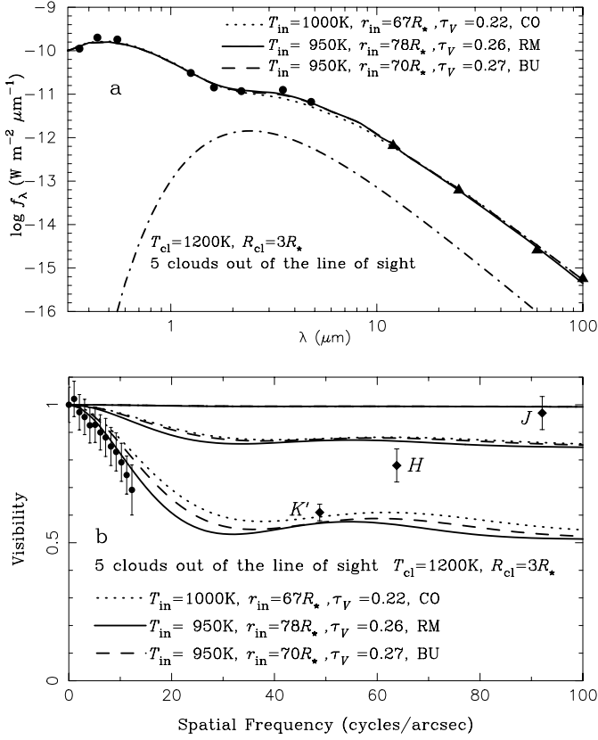
Fig. 4. Comparison of the observed SED and visibilities with SEDs and visibilities predicted by models consisting of the central star, an optically thin dust shell, and a group of five newly formed dust clouds, as shown in Fig. 3. The dashed-dotted line in a ) represents the contribution of the group of newly formed dust clouds in the RM model. See also the legend to Fig. 2.
