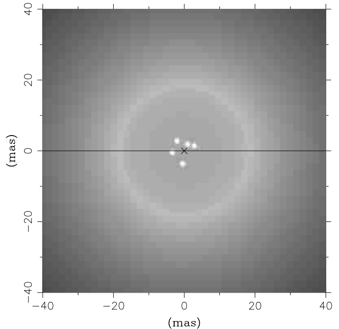
Fig. 3. An example of the intensity distribution of a model with a group of dust clouds, which are randomly distributed at distances of between 2 R_\star and 20 R_\star in the plane of the sky. The intensity is represented in a logarithmic grayscale, where the brighter gray corresponds to the higher intensity. The five intensity peaks located near the central star ( \times ) correspond to newly formed dust clouds. The ring-shaped intensity distribution results from limb brightening of the inner boundary of the optically thin dust shell at 78 R_\star (18 mas). The projected baseline used in the calculation of the visibilities is shown by the solid line.
