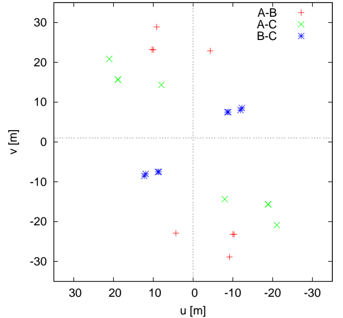
Fig. 2. uv -plane coverage obtained on \theta^1 Ori D with two IOTA array configurations. Symbols and colors as in Figure 1.
